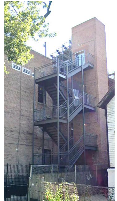
1050 Waveland Ave - Chicago – Structural engineering design of new roof top bleachers across from Wrigley Field. Engineering design included reinforcing the existing building for support of bleacher system, new roof framing and new elevator / stair tower for direct rooftop access.
